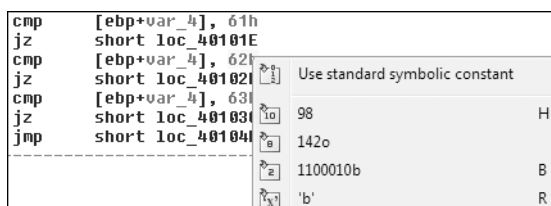
Figure 5-10: Function operand manipulation
