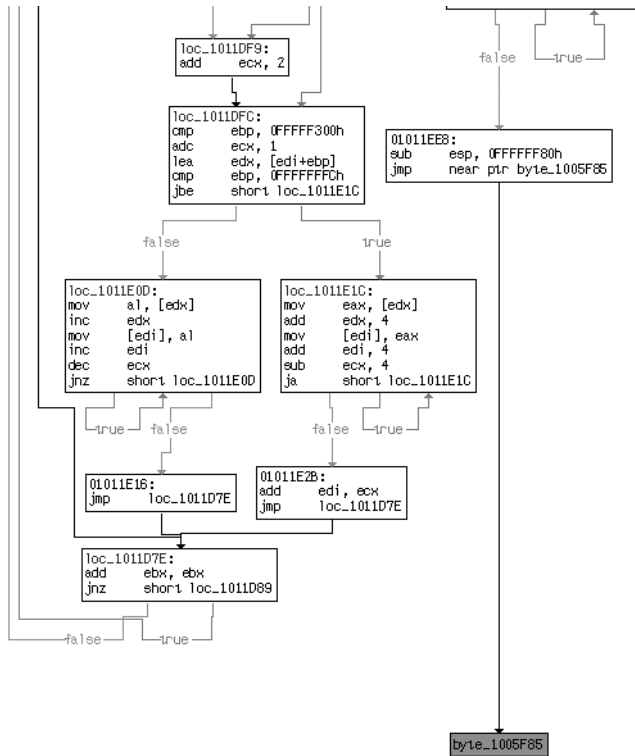
Figure 18-5: A tail jump is highlighted in red in the IDA Pro graph view.
