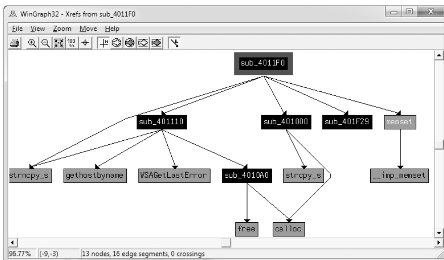
Figure 5-9: Cross-reference graph of a single function (sub_4011F0)
