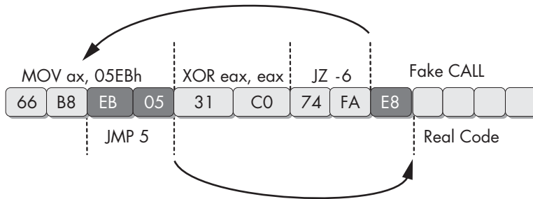
Figure 15-5: Multilevel inward-jumping sequence
