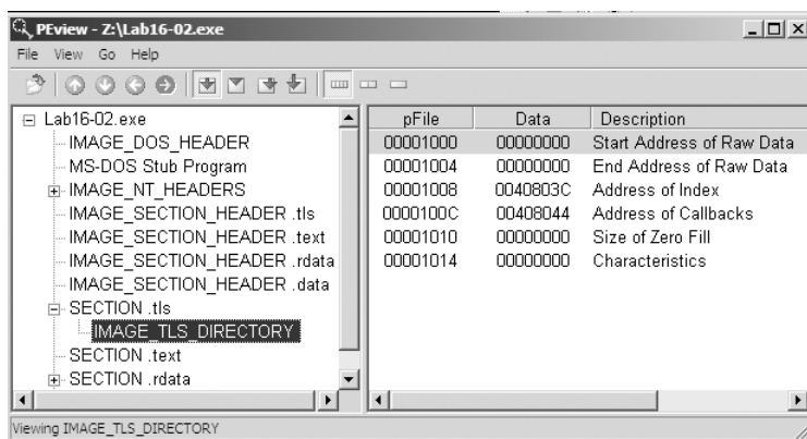
Figure 16-4L: PEView displaying a TLS section for Lab 16-2
