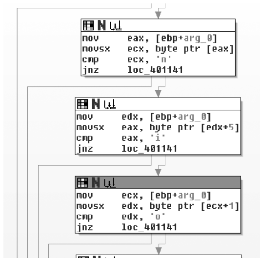
Figure 14-41: Obfuscated string comparison
