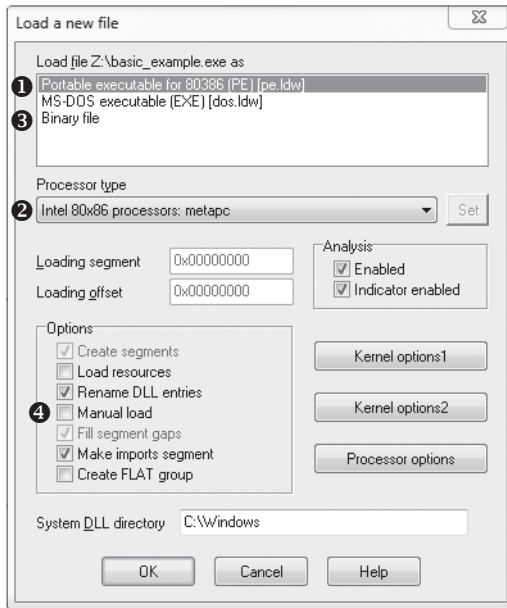
Figure 5-1: Loading a file in IDA Pro
