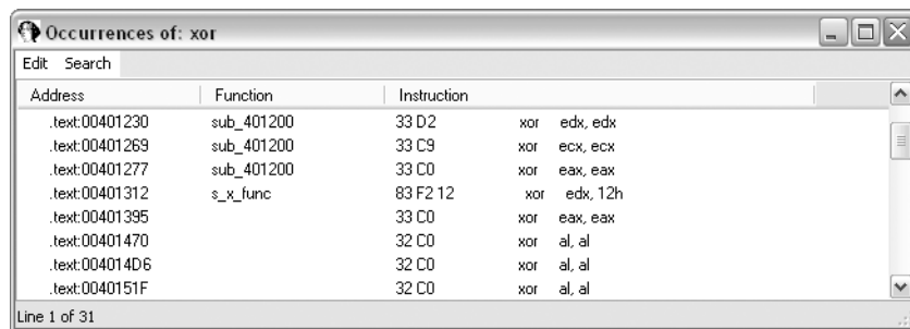
Figure 13-2: Searching for XOR in IDA Pro
