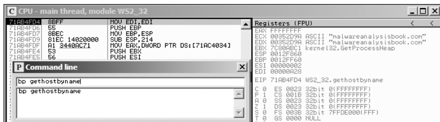
Figure 9-17: Using the command line to quickly set breakpoints
