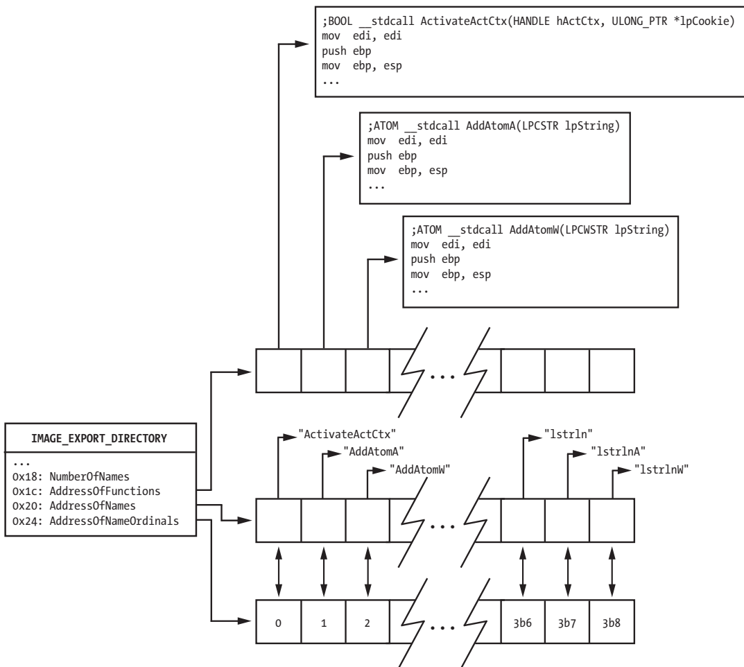
Figure 19-2: kernel32.dll IMAGE_EXPORT_DIRECTORY
