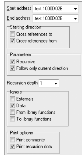
Figure 5-5L: Dialog for setting a custom cross-reference graph from 0x1000D02E
