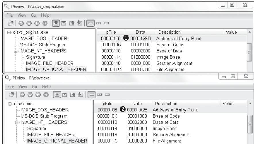
Figure 11-7L: PEvent of original and trojanized versions of cisvc.exe
