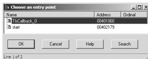
Figure 16-5L: PEView displaying a TLS section for Lab 16-2
