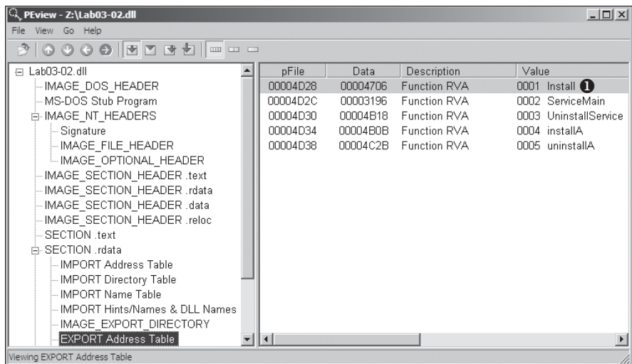
Figure 3-5L: PEView of Lab03-02.dll exports
