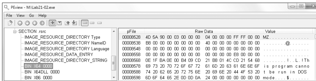
Figure 21-2L: PEview showing three different resource sections
