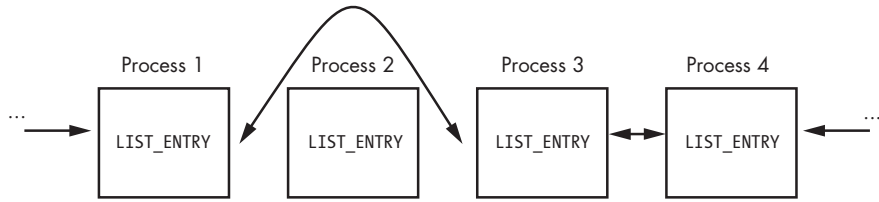
Figure 10-3L: A process being removed from the process list so that it's hidden from tools such as Task Manager
