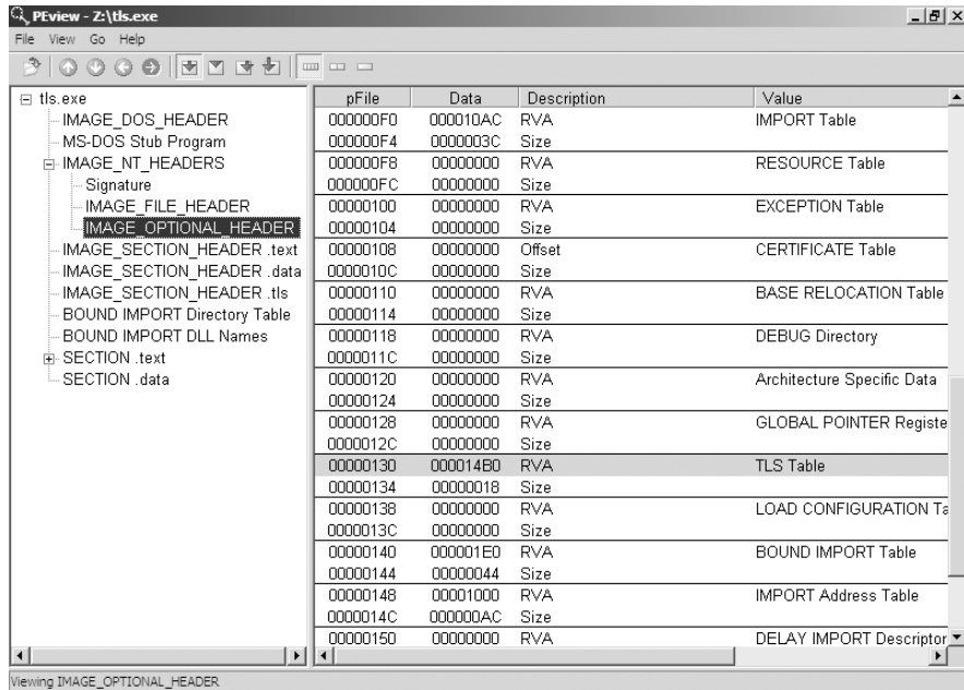
Figure 16-1: TLS callback example—a TLS table in PEView
