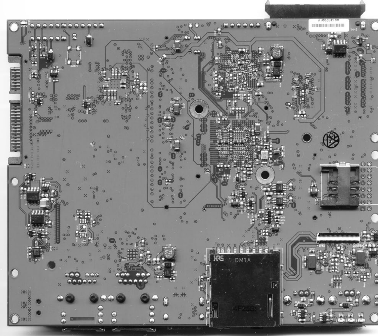
The updated Novena motherboard
