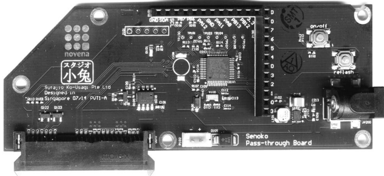
The desktop's pass-through board
