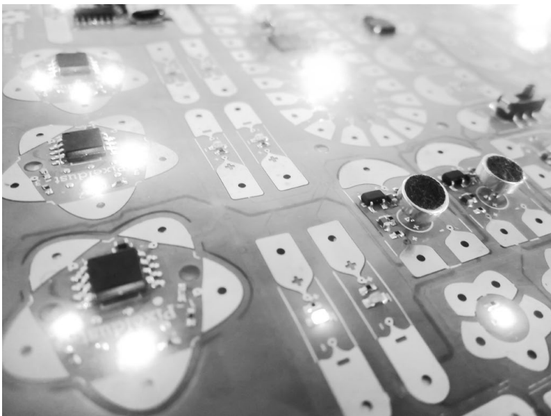
The circuit sticker design we manufactured for the process capability test
