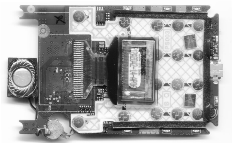
Everything from the display to the battery is soldered directly to the board.
