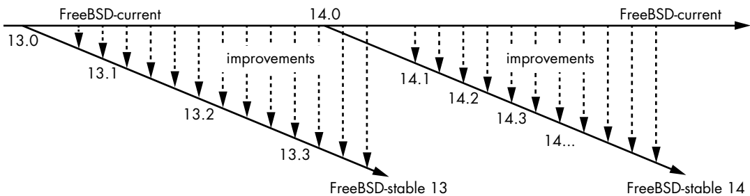
Figure 18-1: FreeBSD development branches
