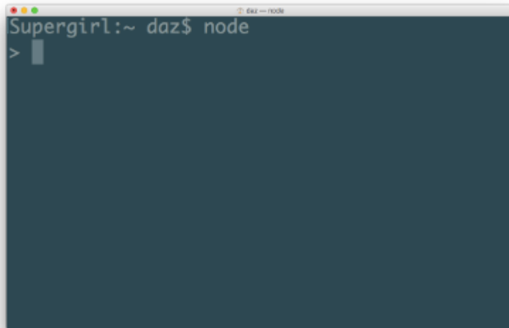
1-1. The REPL
