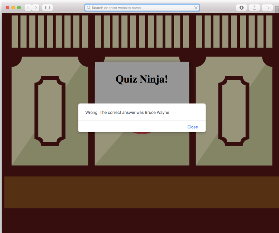
4-1. Quiz Ninja
