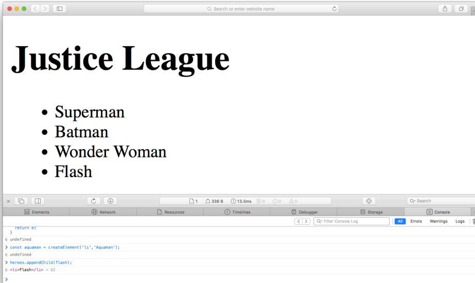
6-6. Append child
