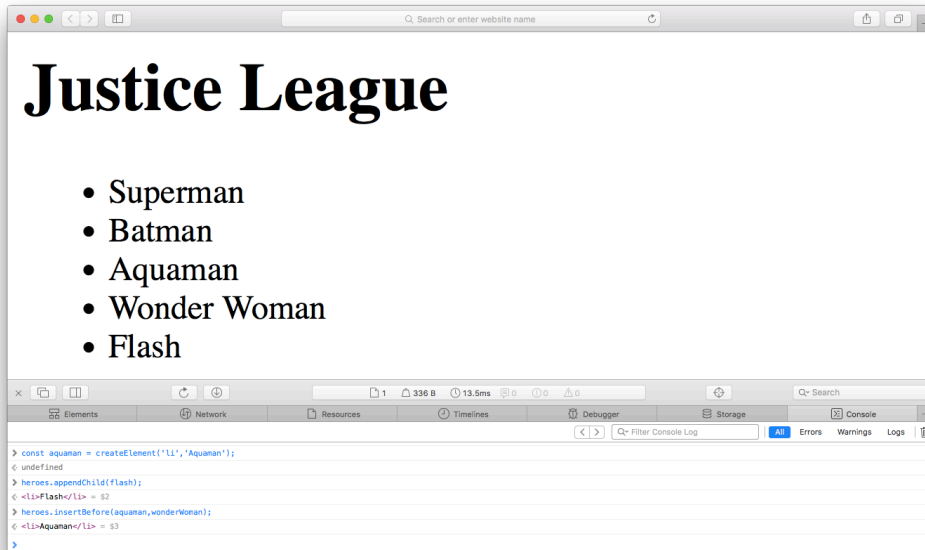
6-7. Insert before
