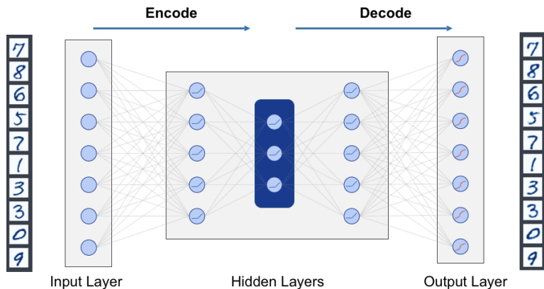
Figure 20.1: Undercomplete encoder-decoder architecture
