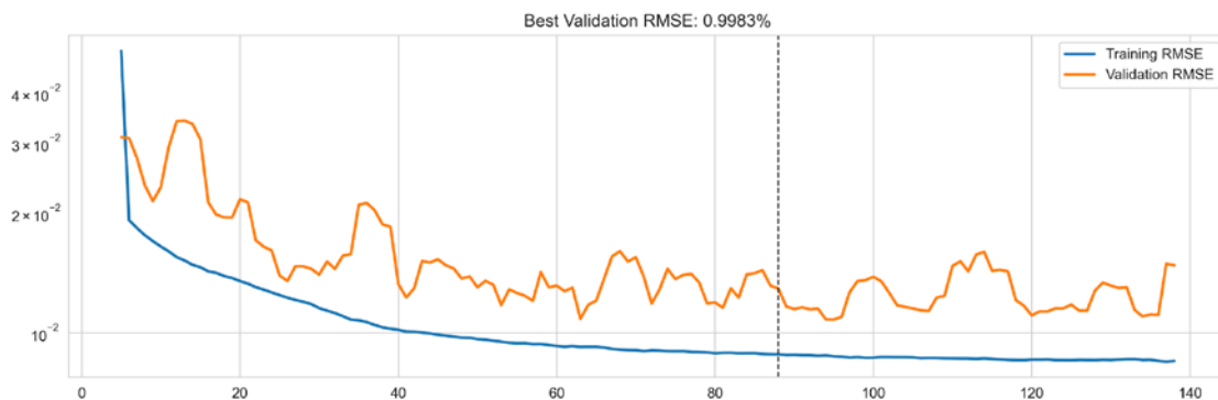
Figure 19.7: Cross-validation performance
