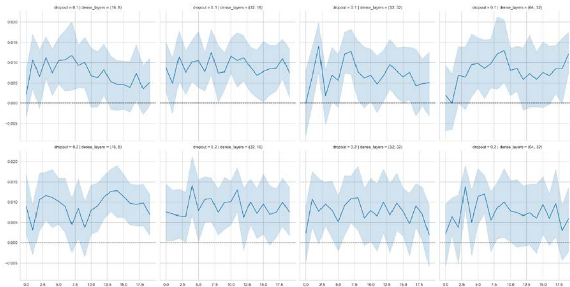
Figure 17.7: Information coefficients for various model configurations
