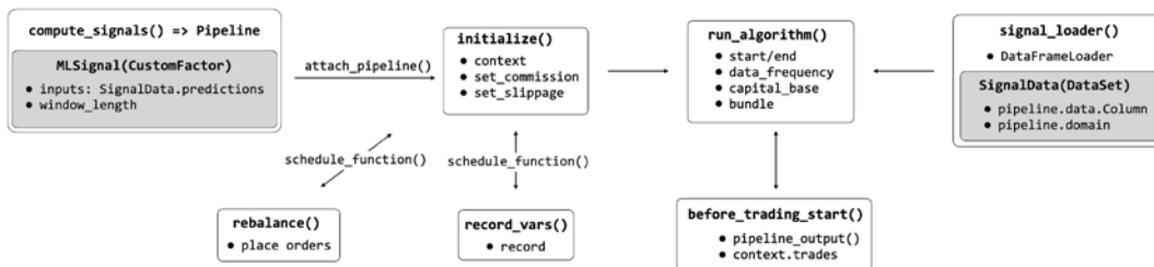
Figure 8.6: ML signal backtest using Zipline's Pipeline API
