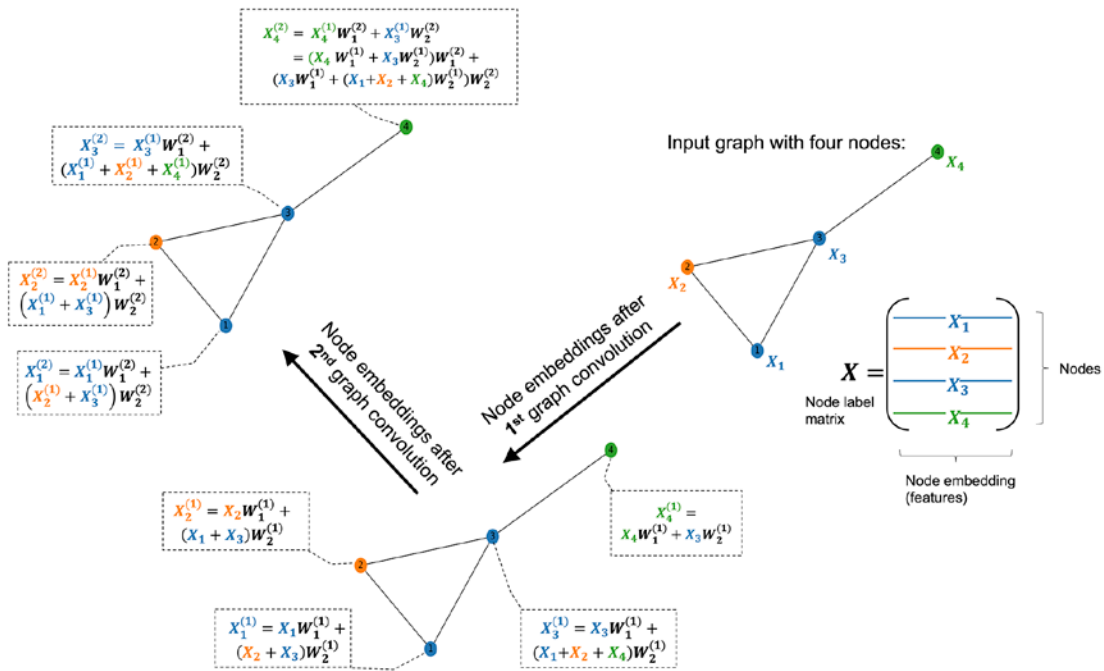
Figure 18.7: Capturing relationships from a graph
