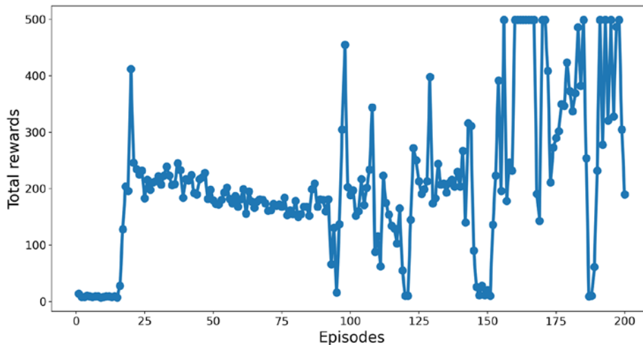
Figure 19.13: The agent's rewards increased over time
