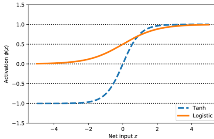
Figure 12.10: A comparison of the tanh and logistic functions
