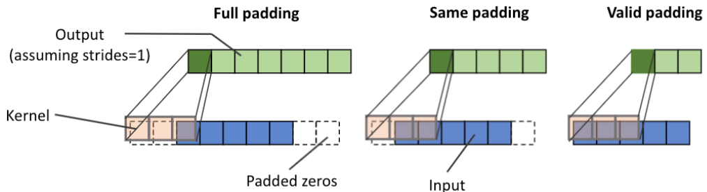
Figure 14.4: The three modes of padding
