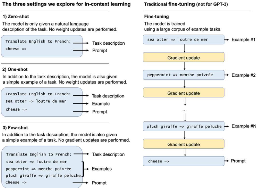
Figure 16.12: A comparison of zero-shot, one-shot, and few-shot learning
