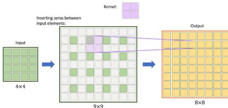
Figure 17.13: Applying transposed convolution to a 4 \times 4 input
