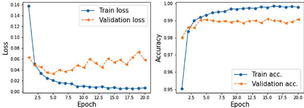
Figure 14.13: Loss and accuracy graphs for the training and validation data
