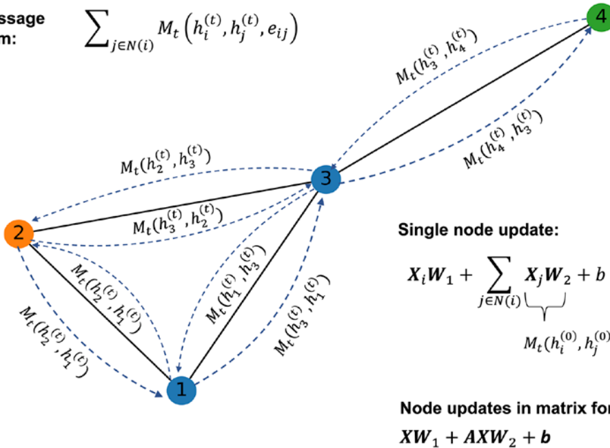
Figure 18.8: The convolutions implemented on the graph and the message form
