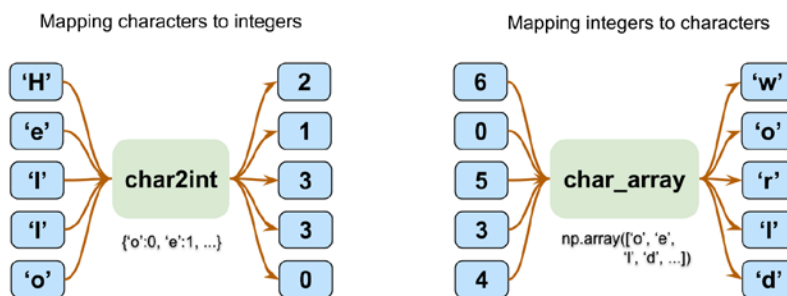
Figure 15.12: Character and integer mappings
