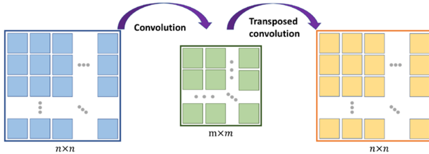
Figure 17.12: Transposed convolution
