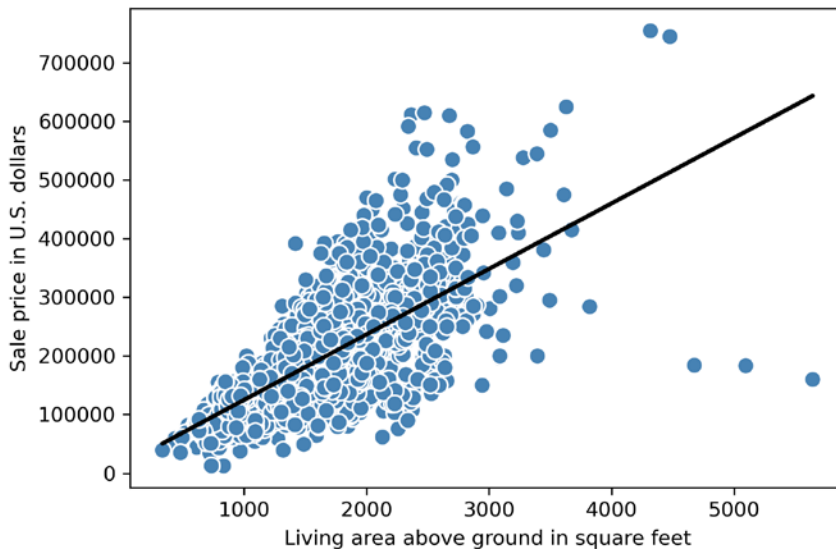
Figure 9.8: A linear regression plot using scikit-learn
