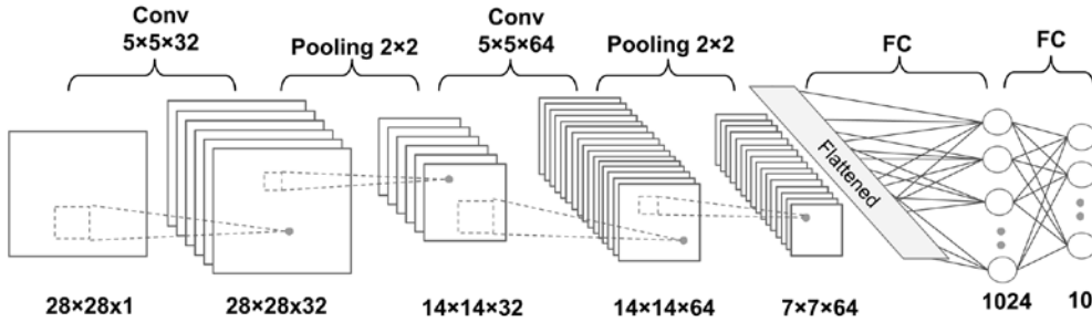
Figure 14.12: A deep CNN
