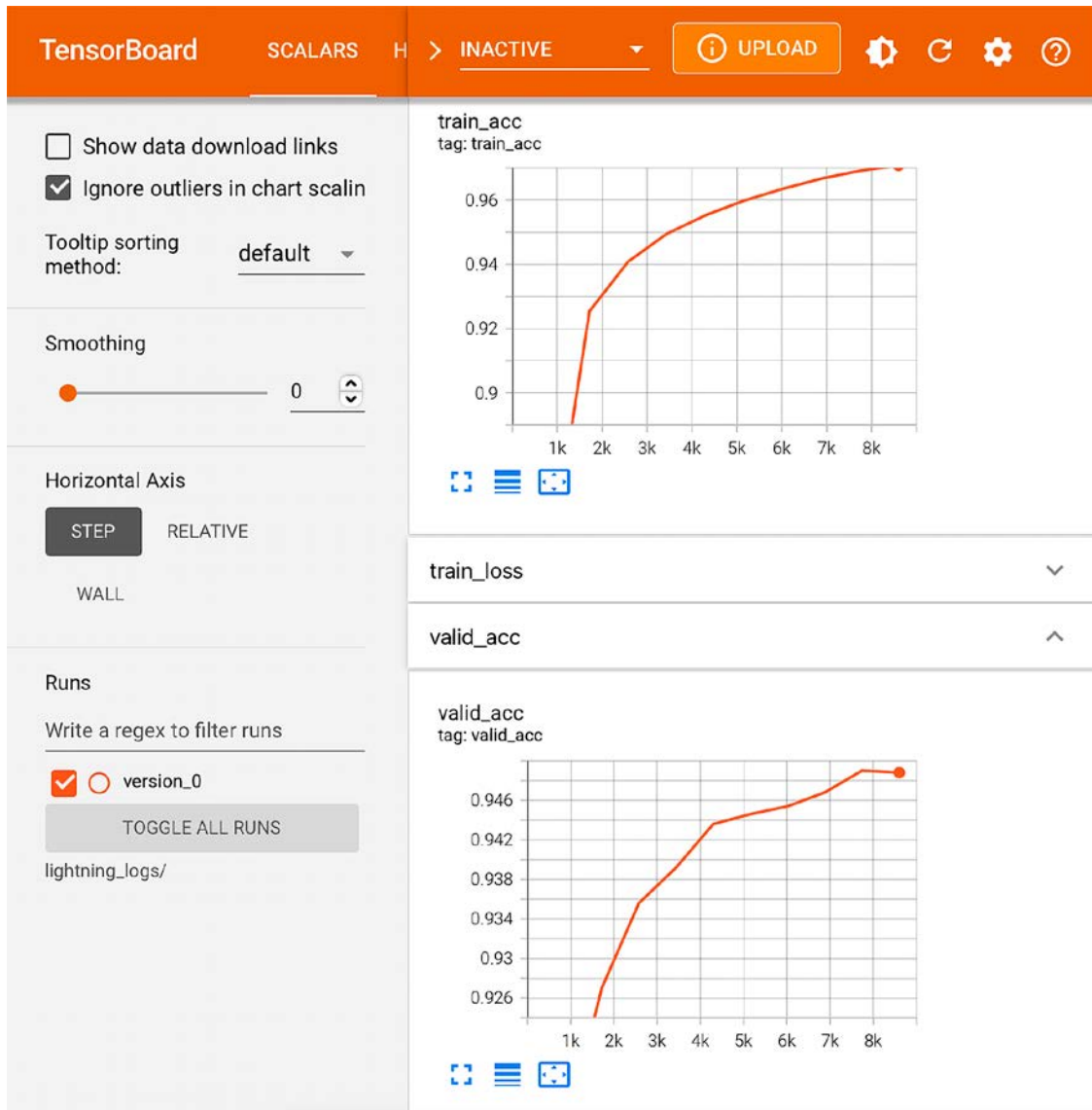
Figure 13.9: TensorBoard dashboard
