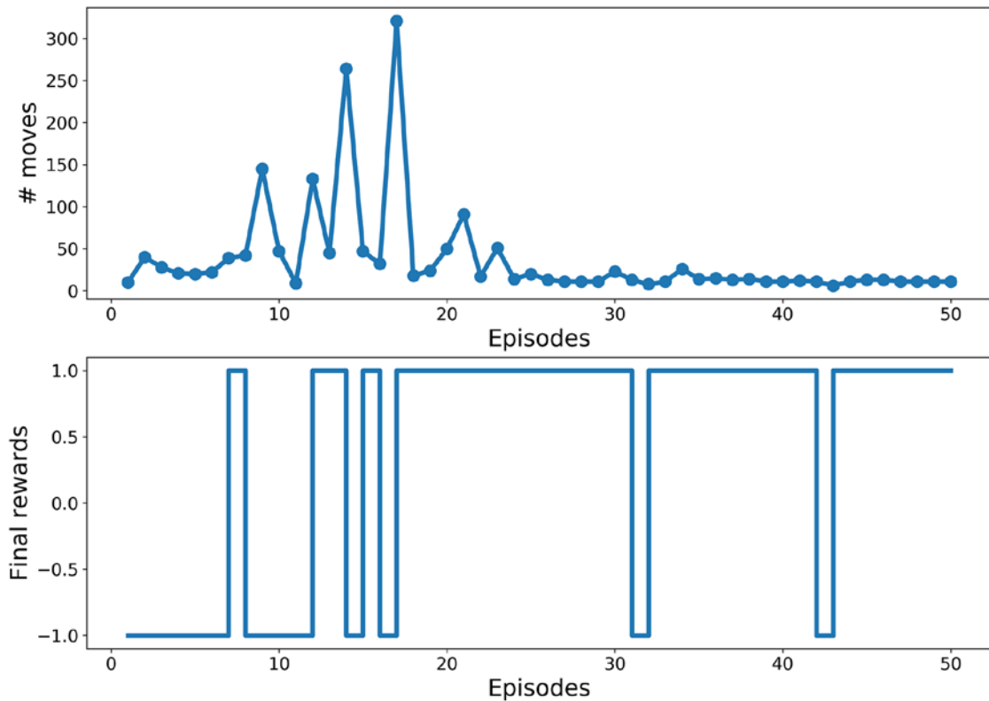
Figure 19.9: The agent's number of moves and rewards
