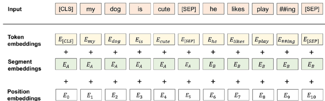
Figure 16.13: Preparing the inputs for the BERT encoder
