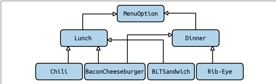
Figure 13-2. A more complicated type hierarchy
