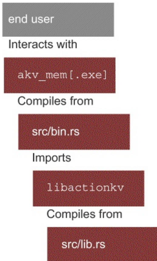
Figure 7.2 Relationship between libactionkv and other components of the actionkv project
