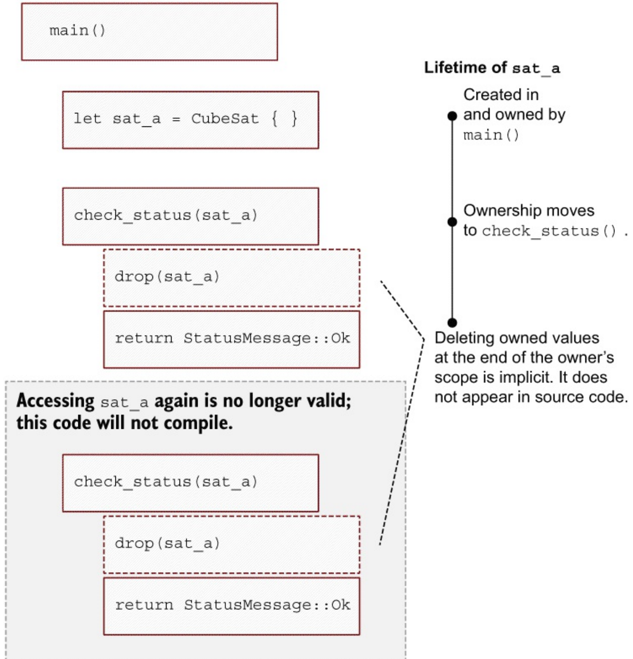
Figure 4.2 Visual explanation of Rust's ownership movement
