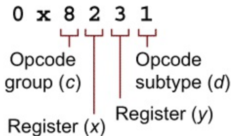
Figure 5.3 CHIP-8 opcodes are decoded in multiple ways. Which to use depends on the value of the leftmost nibble.
