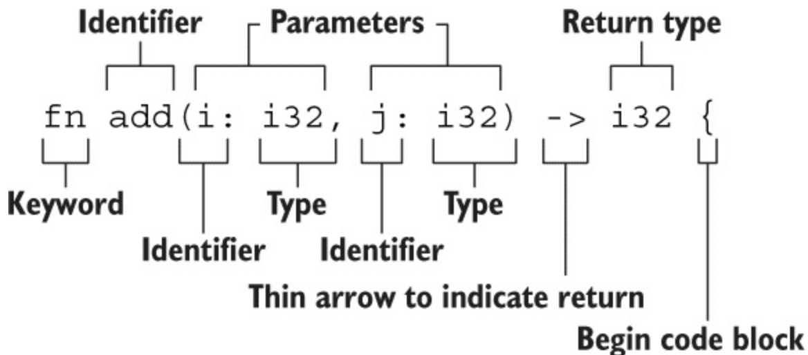
Figure 2.2 Rust's function definition syntax
