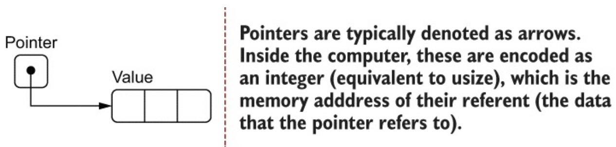
Figure 6.1 Depicting notation used in this chapter's figures for
