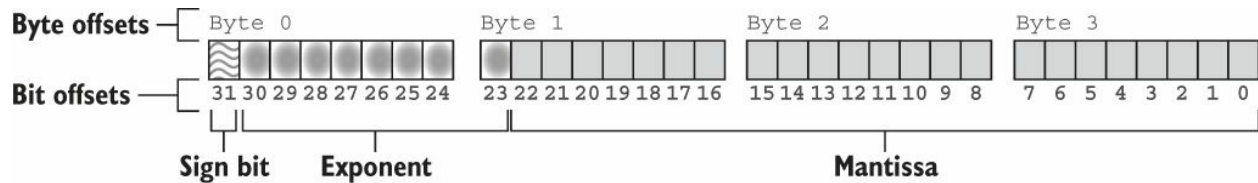
Figure 5.1 An overview of the three components encoded within the bits of a floating-point number for the f32 type in Rust
