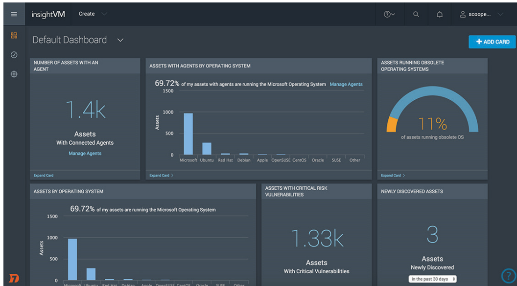
Figure 13.17 – InsightVM
