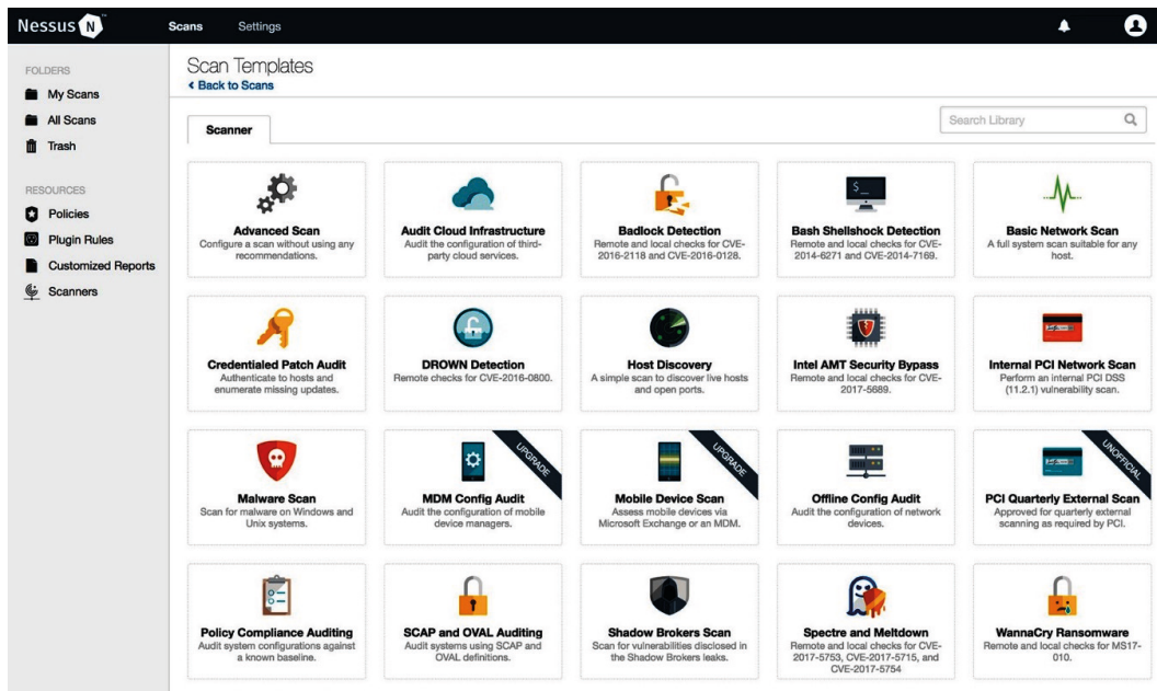
Figure 3.10 – Nessus interface
