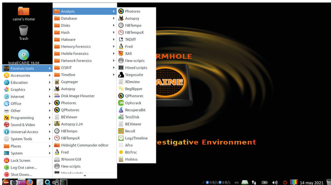
Figure 16.5 – CAINE GUI
