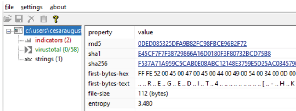
Figure 14.7 – Basic output from PeStudio
