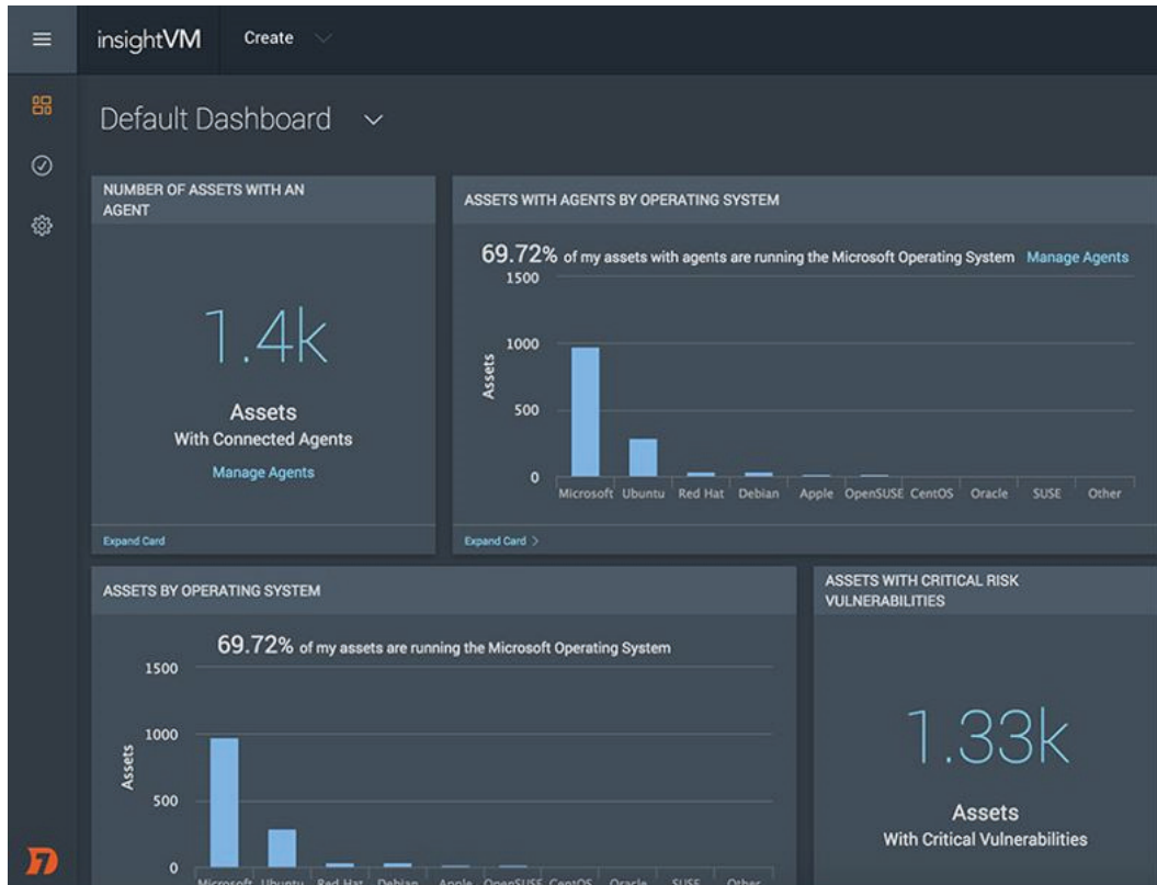
Figure 11.12 – InsightVM Default Dashboard
