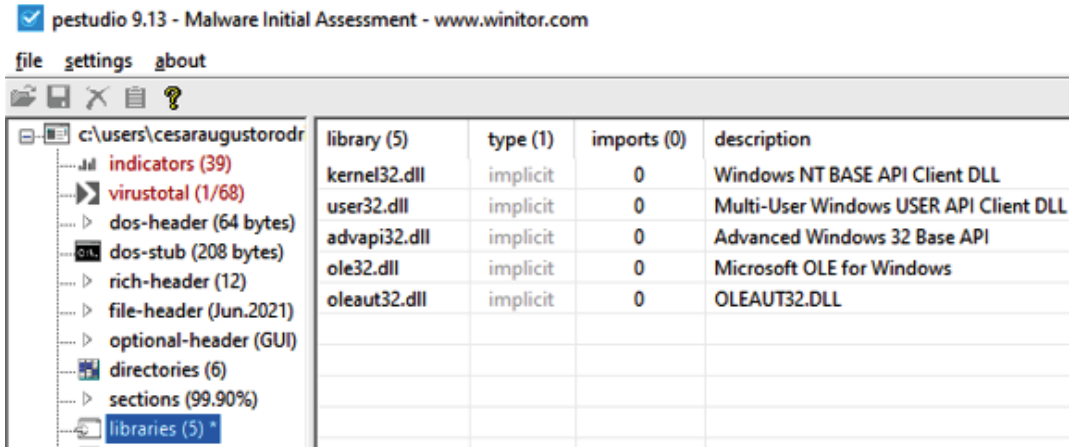
Figure 14.11 – Analysis of libraries on PeStodio
