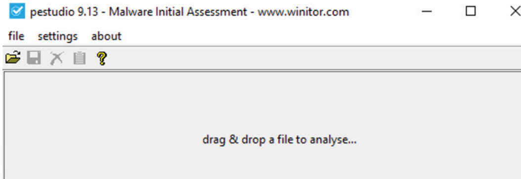
Figure 14.6 – PeStudio GUI
