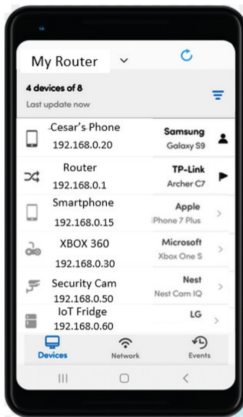
Figure 8.14 – Fing app
