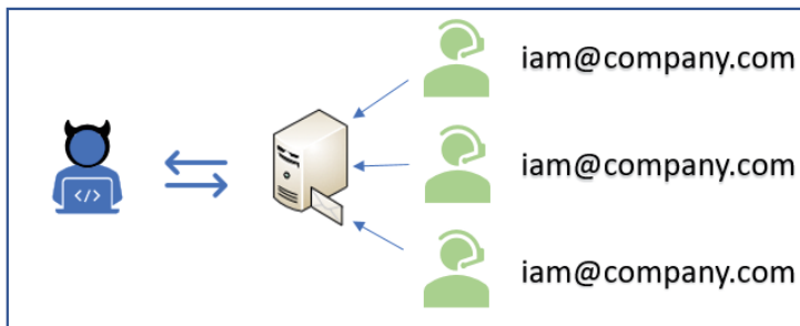
Figure 4.5 – Using mailboxes
