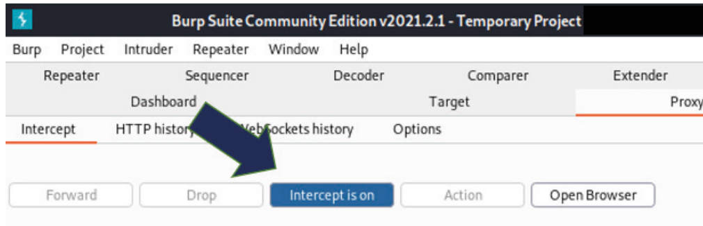
Figure 12.18 – Turning on Intercept in Burp Suite
