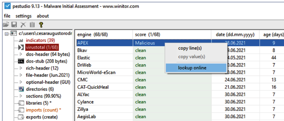
Figure 14.12 – View of VirusTotal scan results on PeStodio
