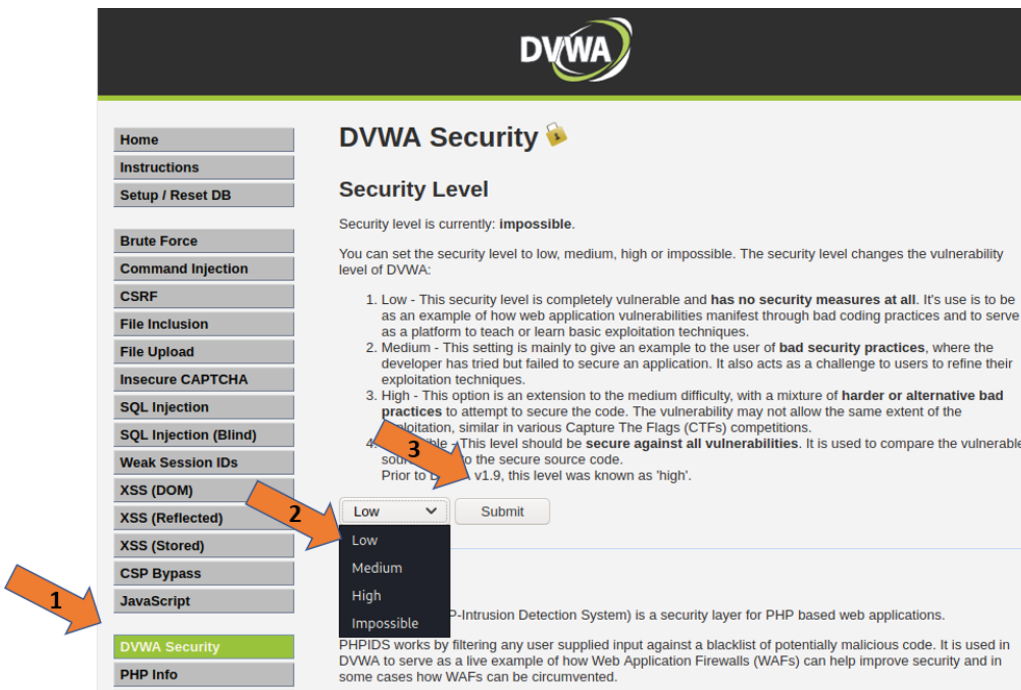
Figure 15.22 – Lowering the security level in DVWA
