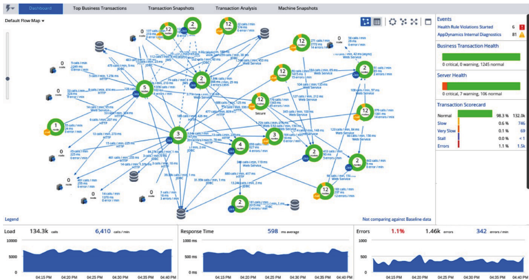
Figure 11.10 – AppDynamics
