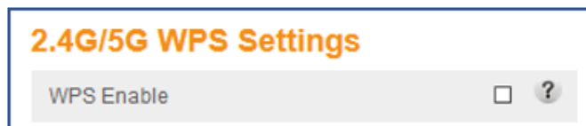
Figure 8.12 – WPS settings
