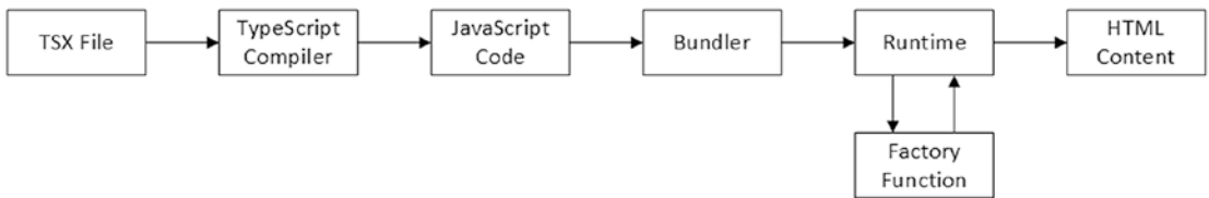
Figure 15-6. Transforming JSX
