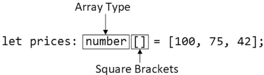
Figure 9-1. An array type annotation
