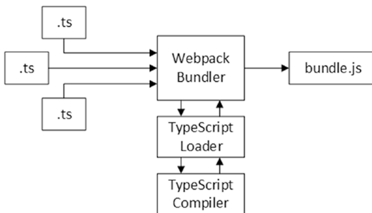
Figure 15-2. Adding a bundle to the toolchain
