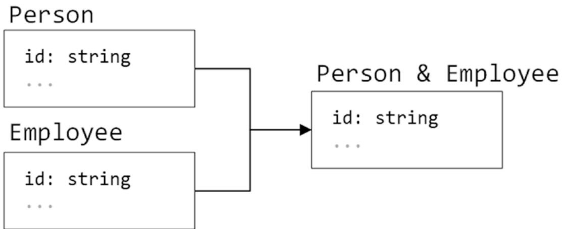
Figure 10-8. Merging properties with the same type
