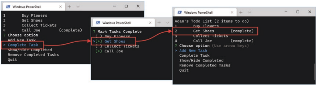
Figure 1-5. Completing items
