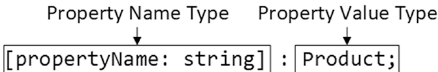
Figure 11-10. An index signature
