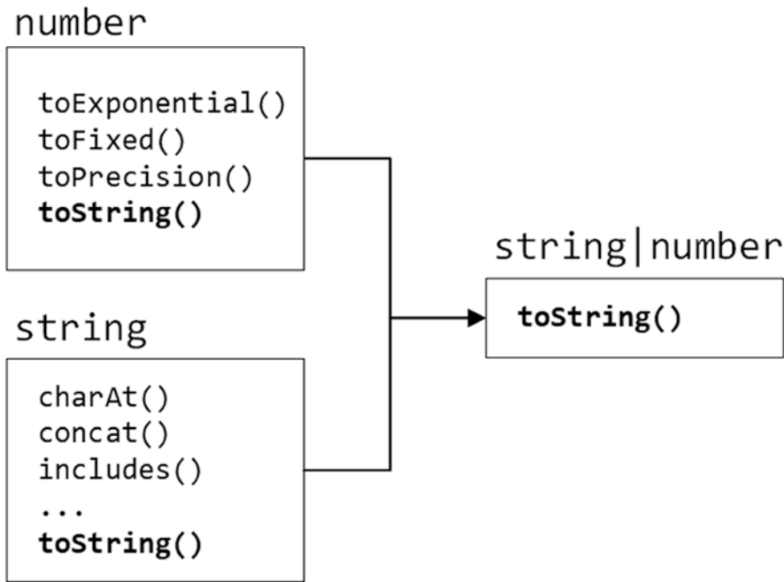
Figure 7-3. The effect of a type union
