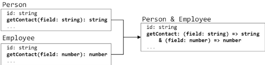
Figure 10-11. Merging methods
