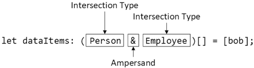
Figure 10-6. Defining an intersection type
