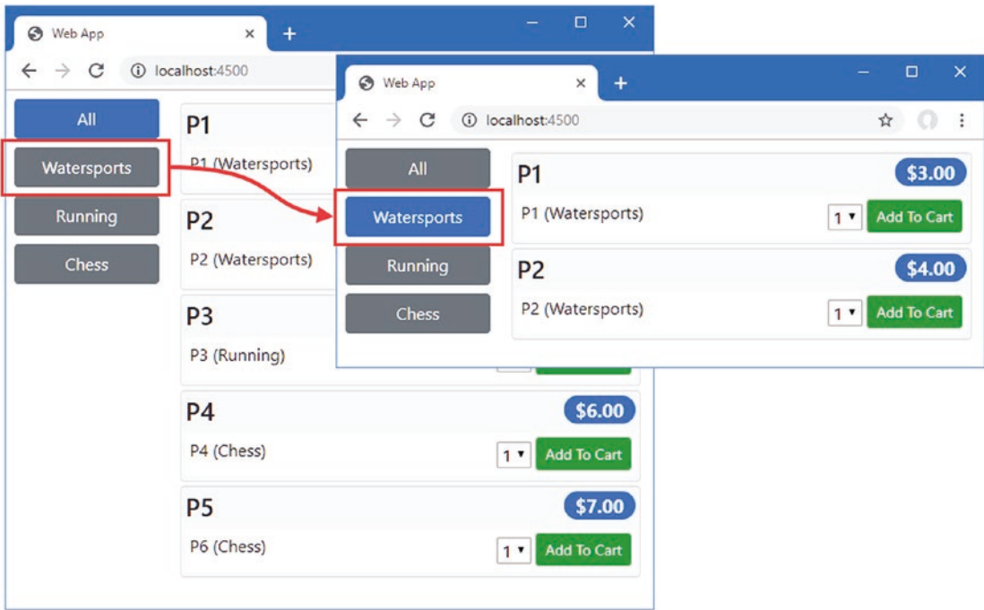
Figure 15-8. Displaying products
