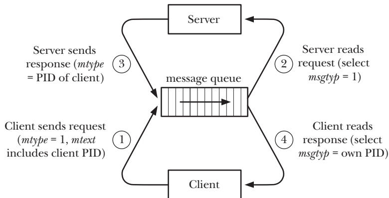
Figure 46-2: Using a single message queue for client-server IPC
