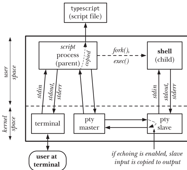
Figure 64-4: The script program
