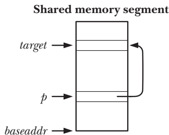
Figure 48-3: Using pointers in a shared memory segment
