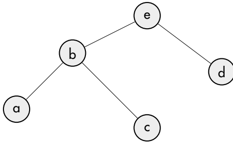
Figure 7-2: Tree
