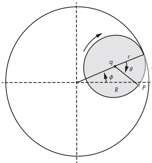
Figure 4-8: Hypocycloid setup
