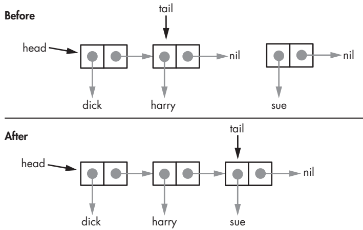
Figure 3-2: Mutable list
