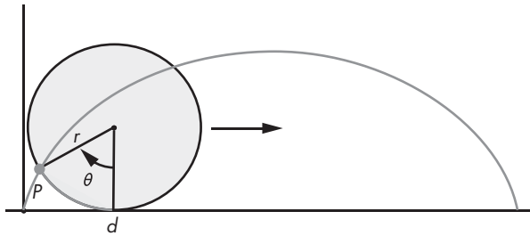
Figure 4-7: Cycloid
