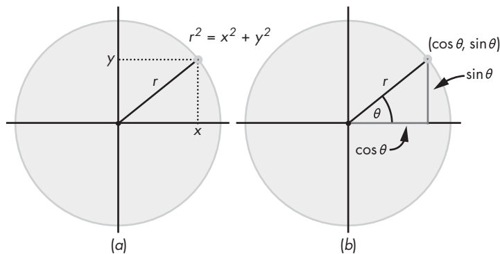
Figure 4-4: Circle definitions
