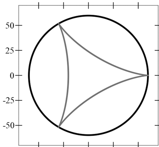
Figure 4-10: Hypocycloid plot
