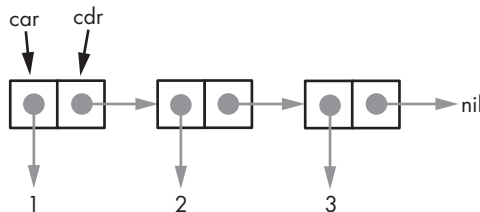
Figure 1-2: List structure
