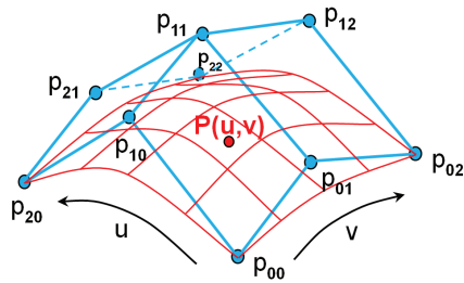
Figure 11.9 Quadratic Bézier control mesh and corresponding surface.
