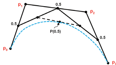
Figure 11.4 Building a cubic Bézier curve.
