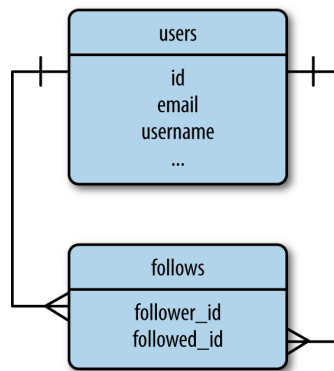
Figure 12-2. Followers, many-to-many relationship
