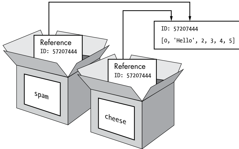
Figure 9-3: cheese[1] = 'Hello!' modifies the list that both variables refer to.
